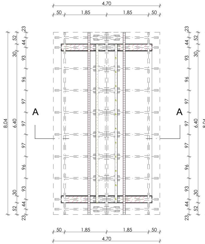
Roof plan
