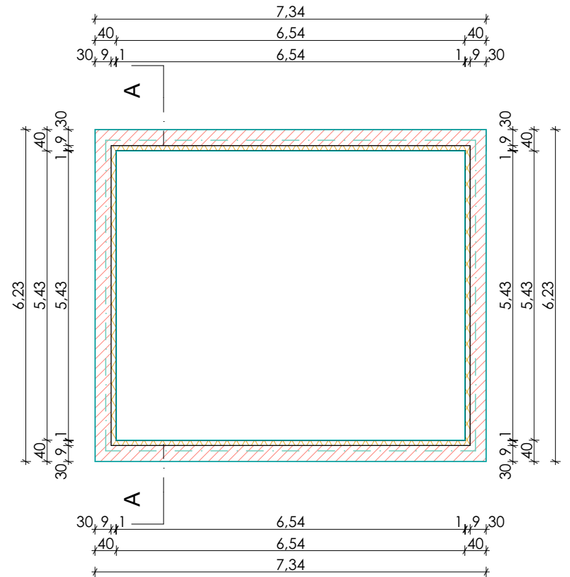
Flat roof with attic wall
