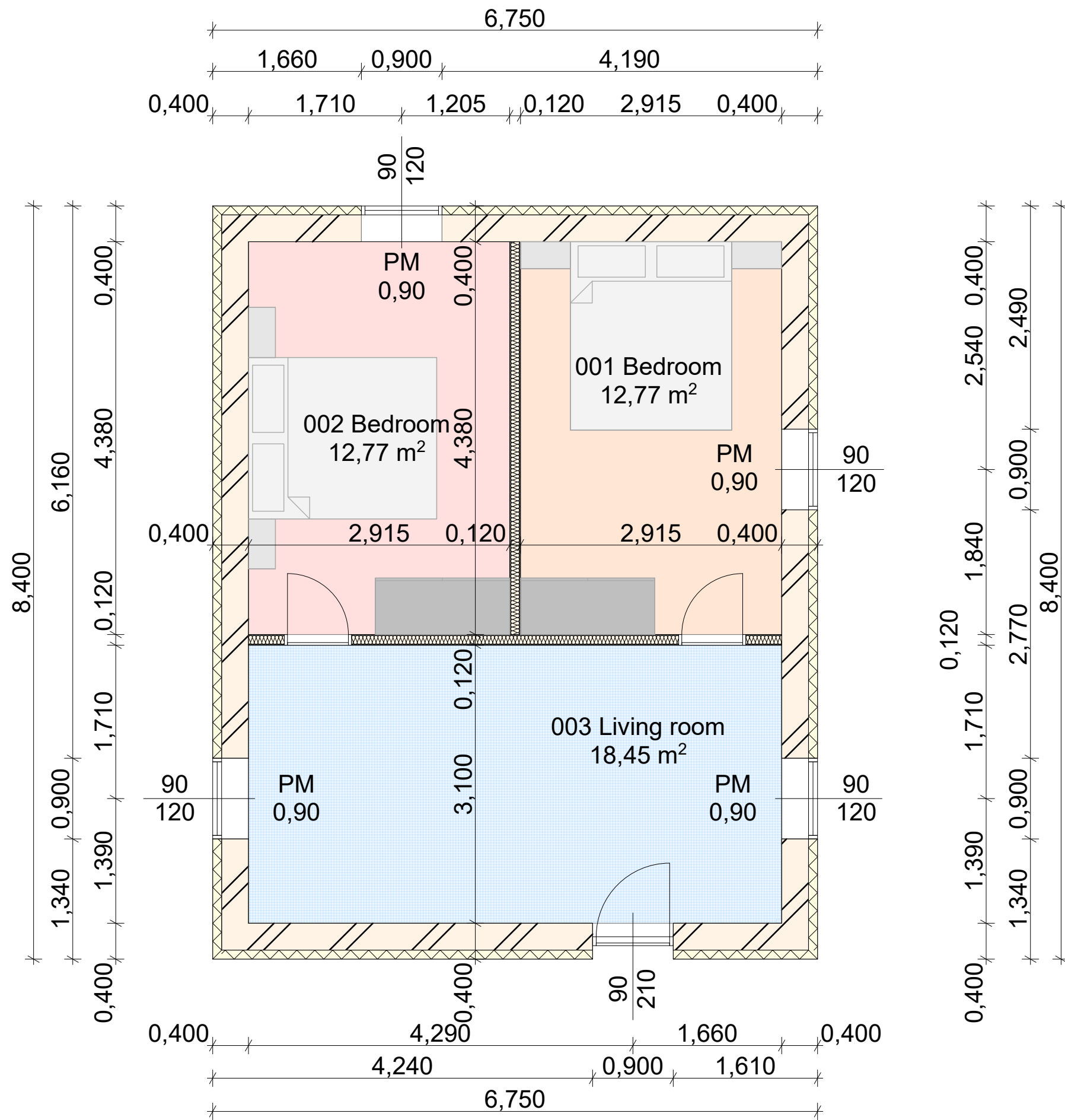
Floor plan 1:50
