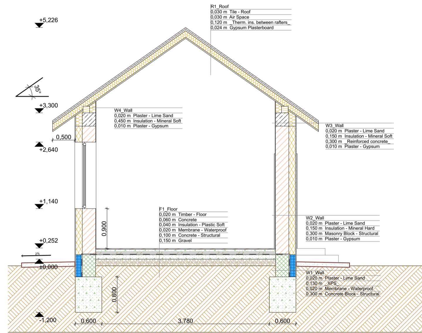
S-01 Section
