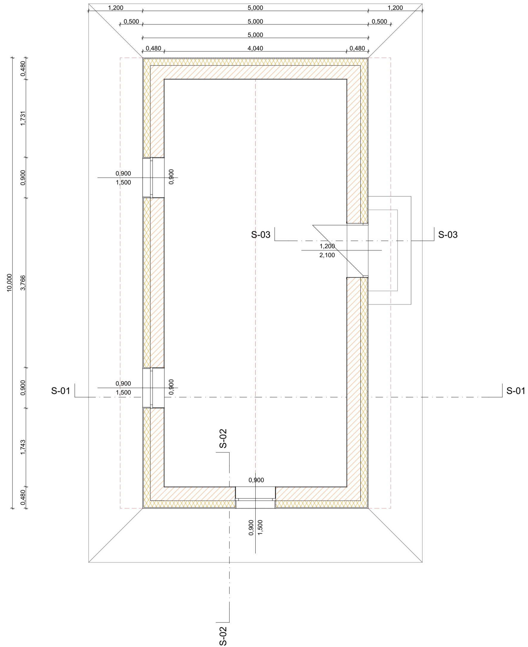
0. Ground floor
